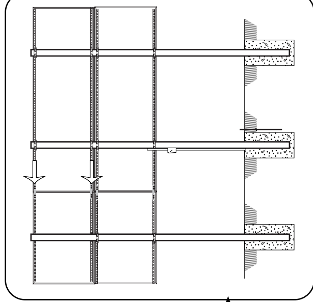
Typical Baseball Multi-Panel Scoreboard Installation Illustration
