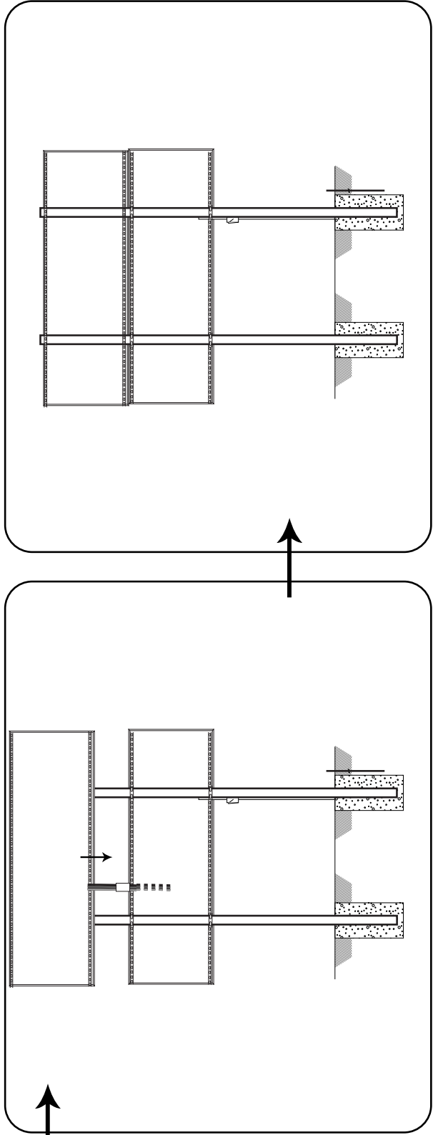
Typical 2 Cabinet Scoreboard Installation Illustration
